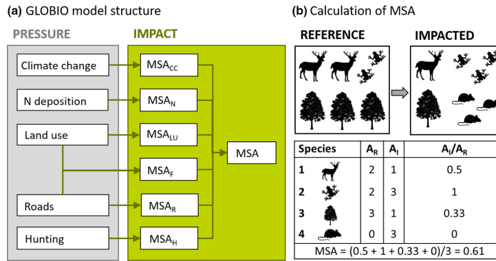
Figure 2: Graphical Summary of the GLOBIO model, Showing (a) the Pressure-Impact Relationships and (b) the Calculation of the MSA Metric
